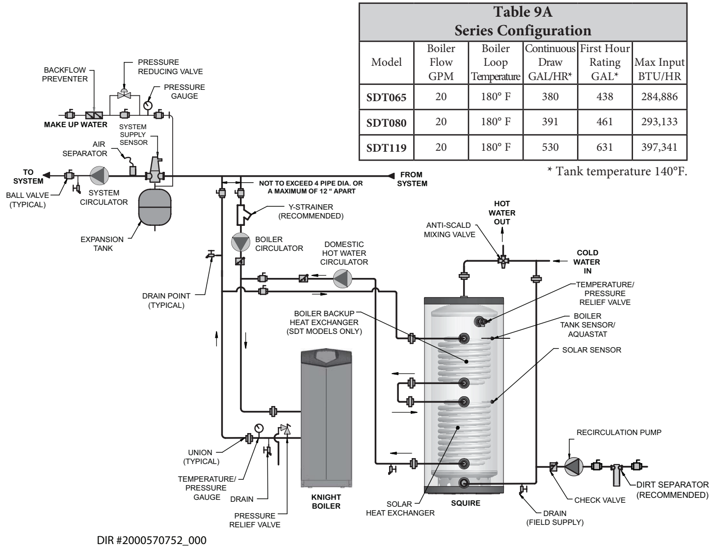
Figure 9-1 Indirect Boiler with Series Piping
