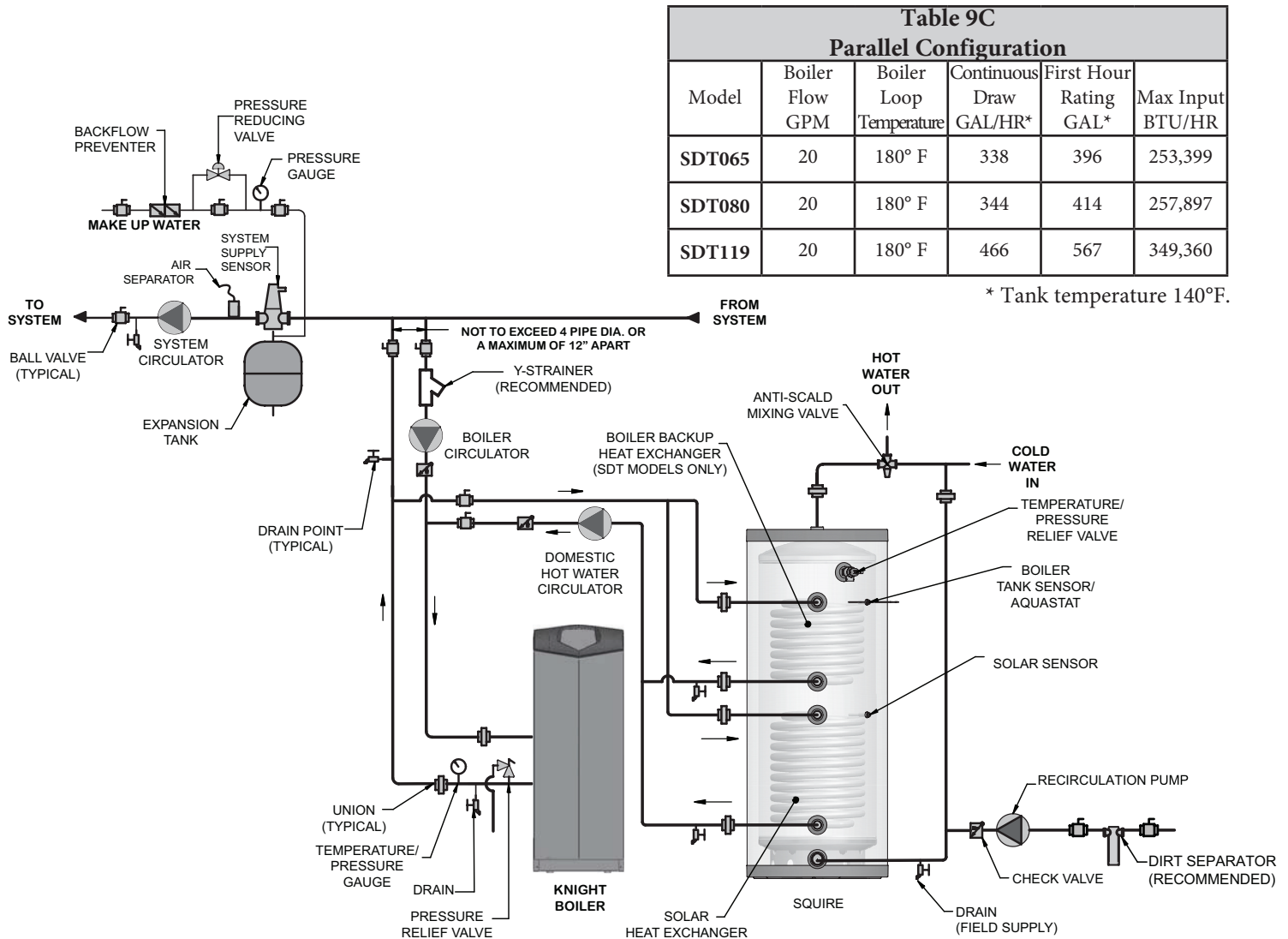
Figure 9-2 Indirect Boiler with Parallel Piping
